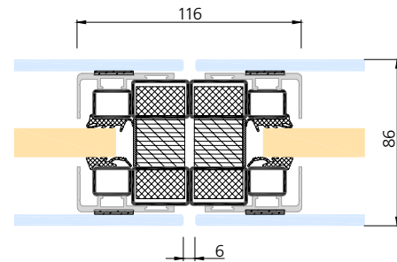
EI30 Verglasung, Tür in Ganzglas-Optik Porte, Cloison EI30 aspect tout verre Door, glazing EI30 all glass design
